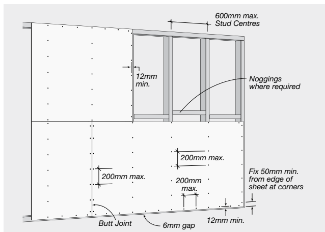
System Overview – Square Edge Wallboard
