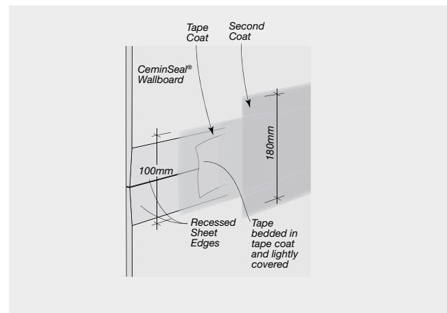
System Overview – Recessed Edge Jointing – Tiled areas
