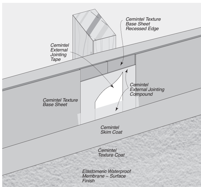
Jointing & Coating System
