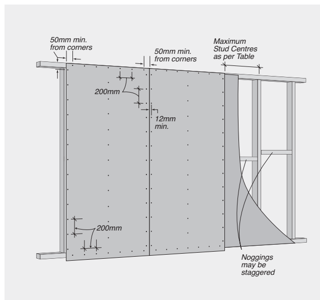
System Overview – Vertical Fixing of Sheets
